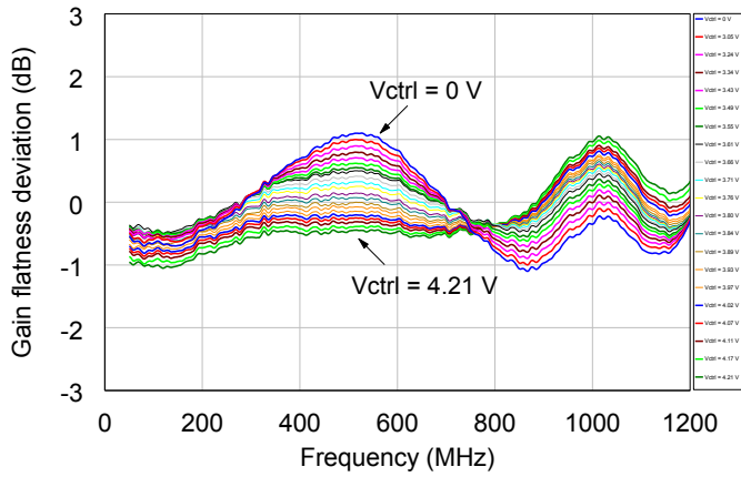
Gain Flatness Deviation @ -40 °C
