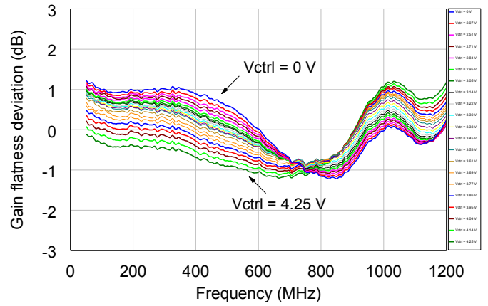
Gain Flatness Deviation @ 85 °C
