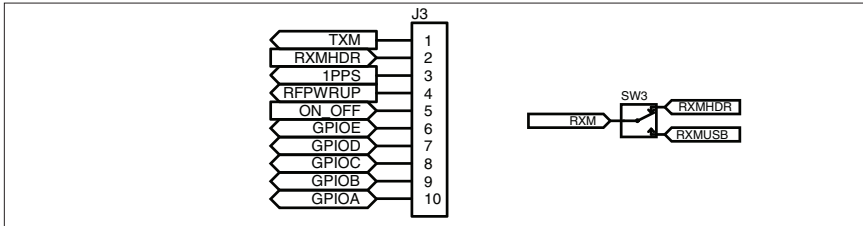
Figure 10: Header Section Schematic
