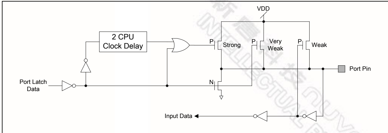
Figure 22-1: Quasi-Bidirectional Output
