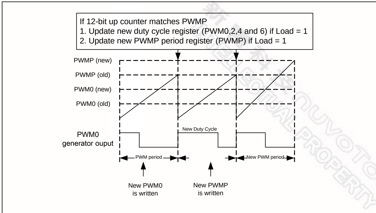
Figure 25-3: Edge-Aligned PWM
