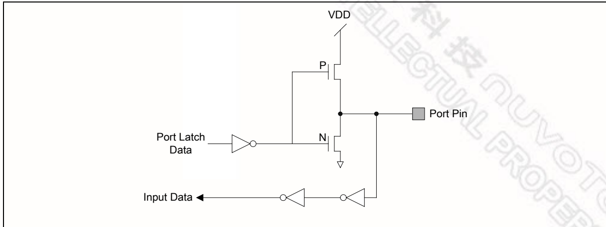
Figure 22-3: Push-Pull Output
