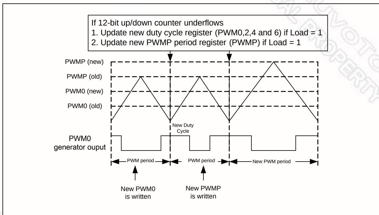
Figure 25-6: Center-Aligned Mode
