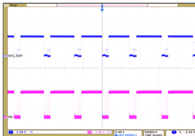
Figure 34 Forced Over Temperature ( V_{IN} = 75V T_{CASE} = 135^{\circ}C I_{OUT} = 27A )
