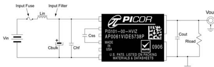
Figure 1 Picor PI3101 Shown With System Fuse, Filter, Decoupling And Extended Soft Start
