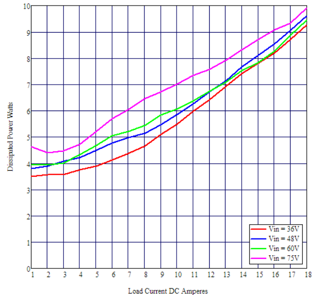
Figure 5 Power Dissipation Vs I_o ( T_{case} = 100^{\circ}C )
