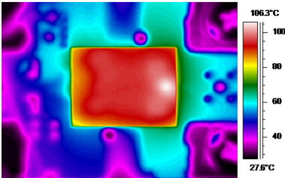
Figure 12 Thermal Image V_{IN} = 48V I_O = 18A Flow = 600LFM Longitudinal No Heat Sink Temp = 25°C
