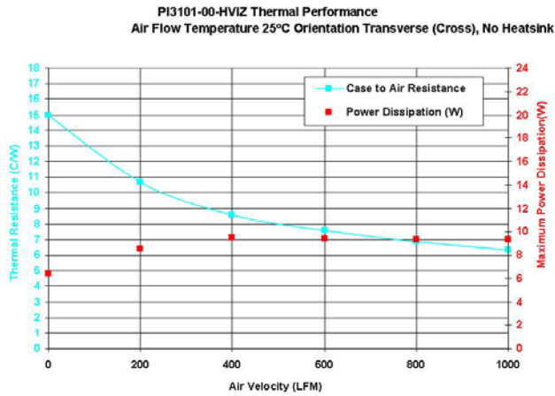
Figure 13 R_{\Theta_{C-A}} (No Heat Sink Transverse Flow)
