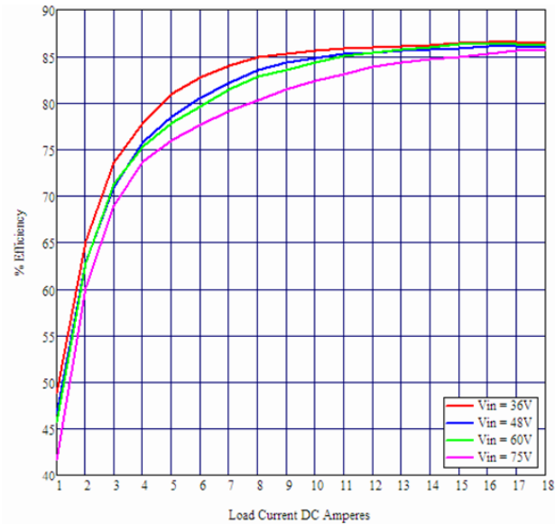
Figure 4 Conversion Efficiency ( T_{case} = 100^{\circ}C )
