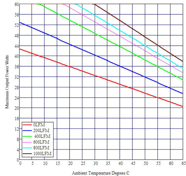
Figure 7 P_{OUT} Vs Temp (No Heat Sink)
