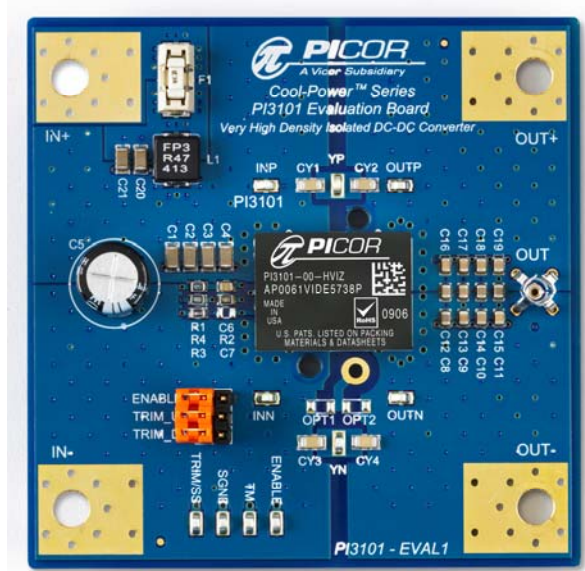
Figure 37 Picor PI3101-EVAL1 Evaluation Board (Actual Size)
