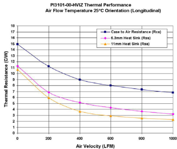
Figure 11 R_{\Theta C-A} (Heat Sinks Longitudinal Flow)
