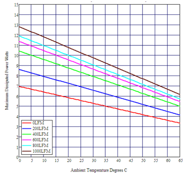
Figure 6 Power Dissipation Vs Temp (No Heat Sink)
