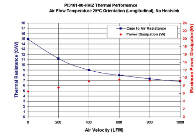
Figure 10 R_{\Theta C-A} (No Heat Sink Longitudinal Flow)
