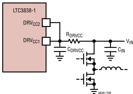
Figure 8. Setup for V IN ≤ 5.3V
