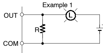
Generating a dark current (about 1/3 of the rated current) through the incandescent bulb.
