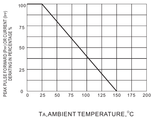
Fig.2 DERATING CURVE
