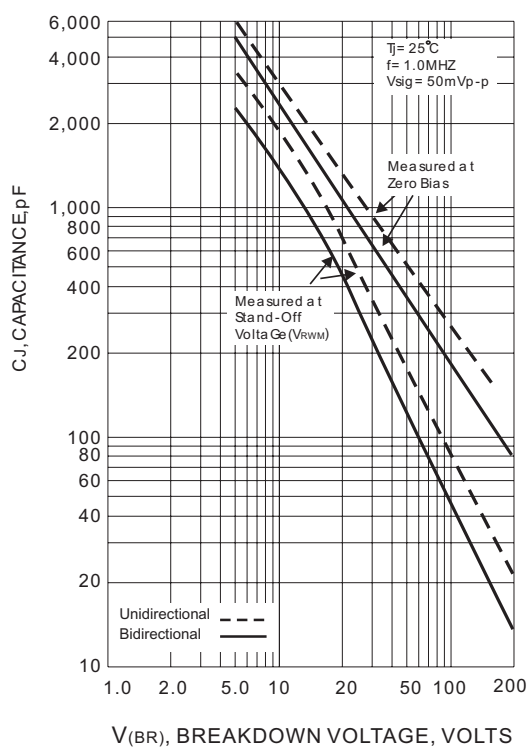
Fig.4 TYPICAL CAPACITANCE
