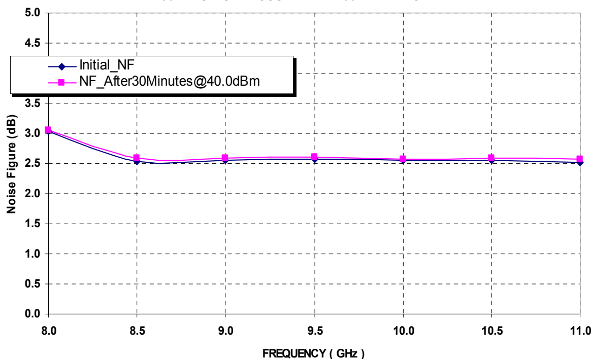
TYPICAL MEASURED NOISE FIGURE OF THE LIMITER/LNA TESTED BEFORE AND AFTER 30 MINUTES EXPOSURE WITH 40dBm CW POWER
