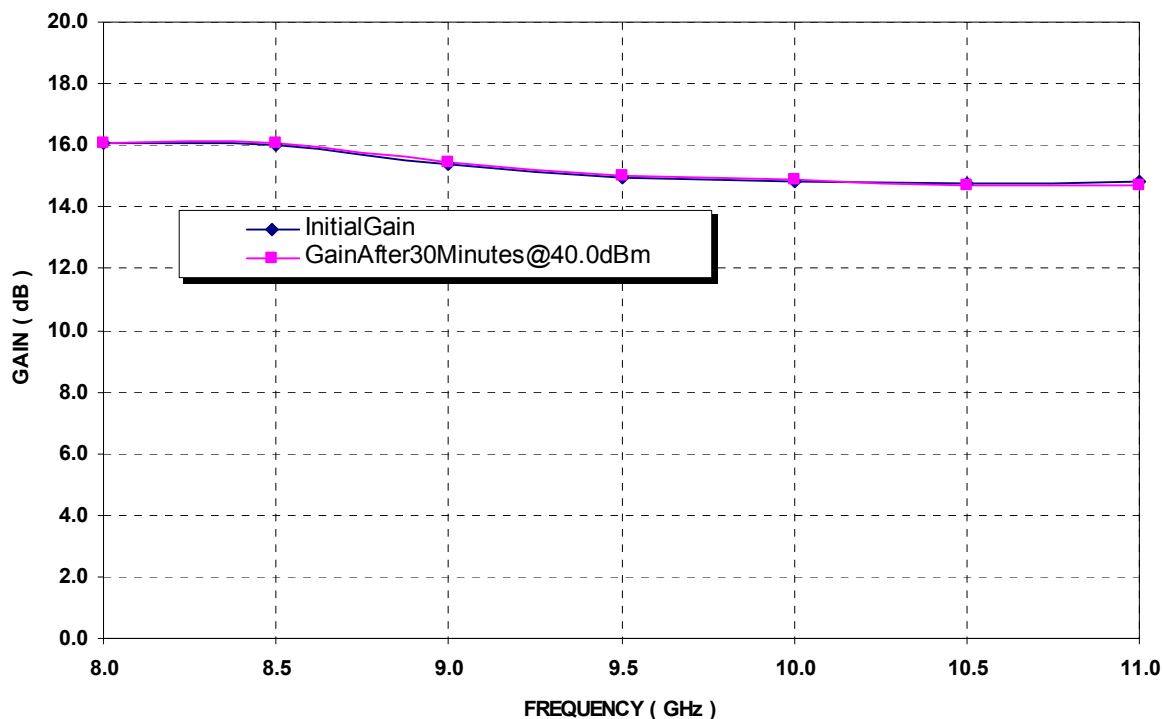
TYPICAL MEASURED GAIN OF THE LIMITER/LNA TESTED BEFORE AND AFTER 30 MINUTES EXPOSURE WITH 40dBm CW POWER
