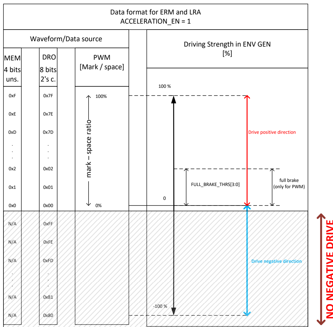
Figure 31: Overview of Data Formats with Acceleration Enabled
