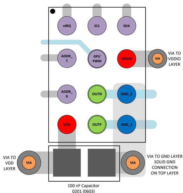
Figure 43: WLCSP Example PCB Layout
