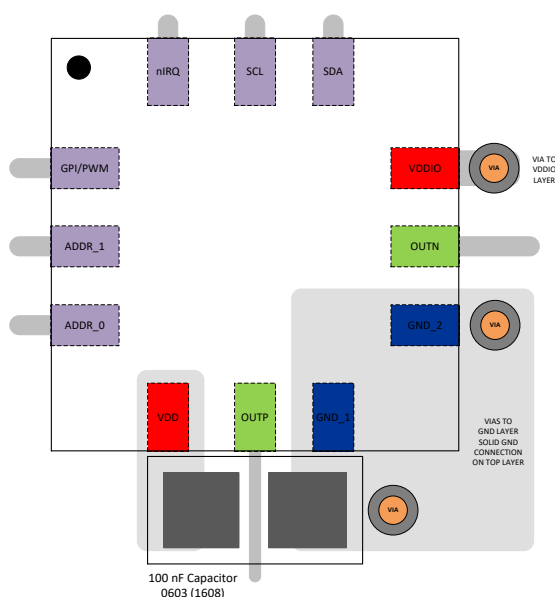
Figure 44: QFN Example PCB Layout
