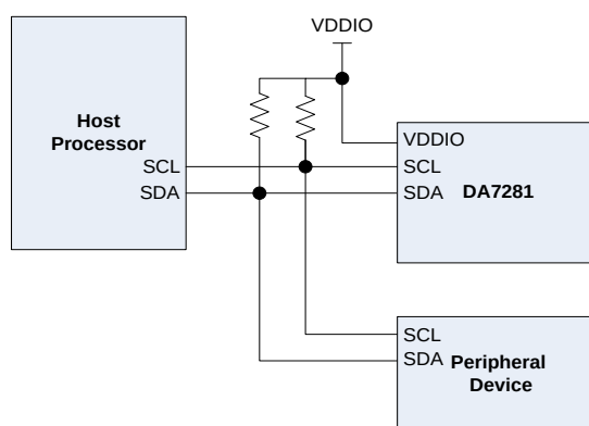
Figure 33: Schematic of the I 2 C Control Interface Bus
