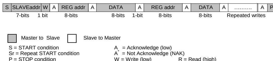
Figure 39: I 2 C Repeated Write (SDA line)
