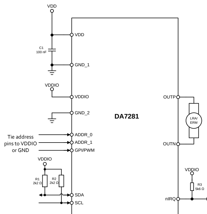
Figure 42: External Components Diagram
