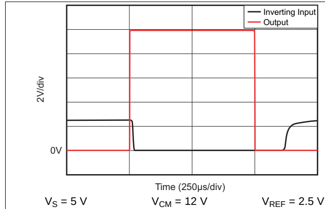
Figure 19. Inverting Differential Input Overload
