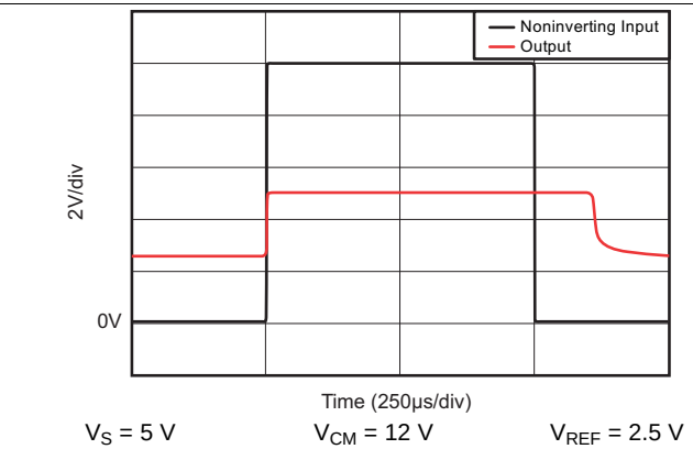
Figure 20. Noninverting Differential Input Overload
