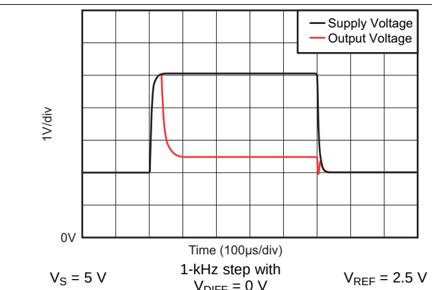
Figure 22. Brownout Recovery
