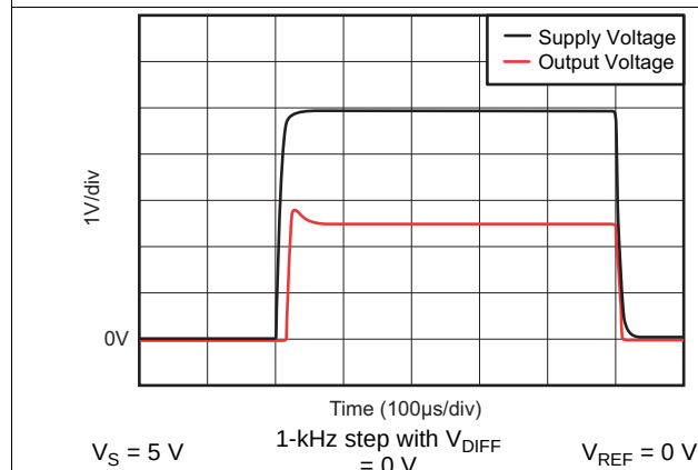
Figure 21. Start-Up Response
