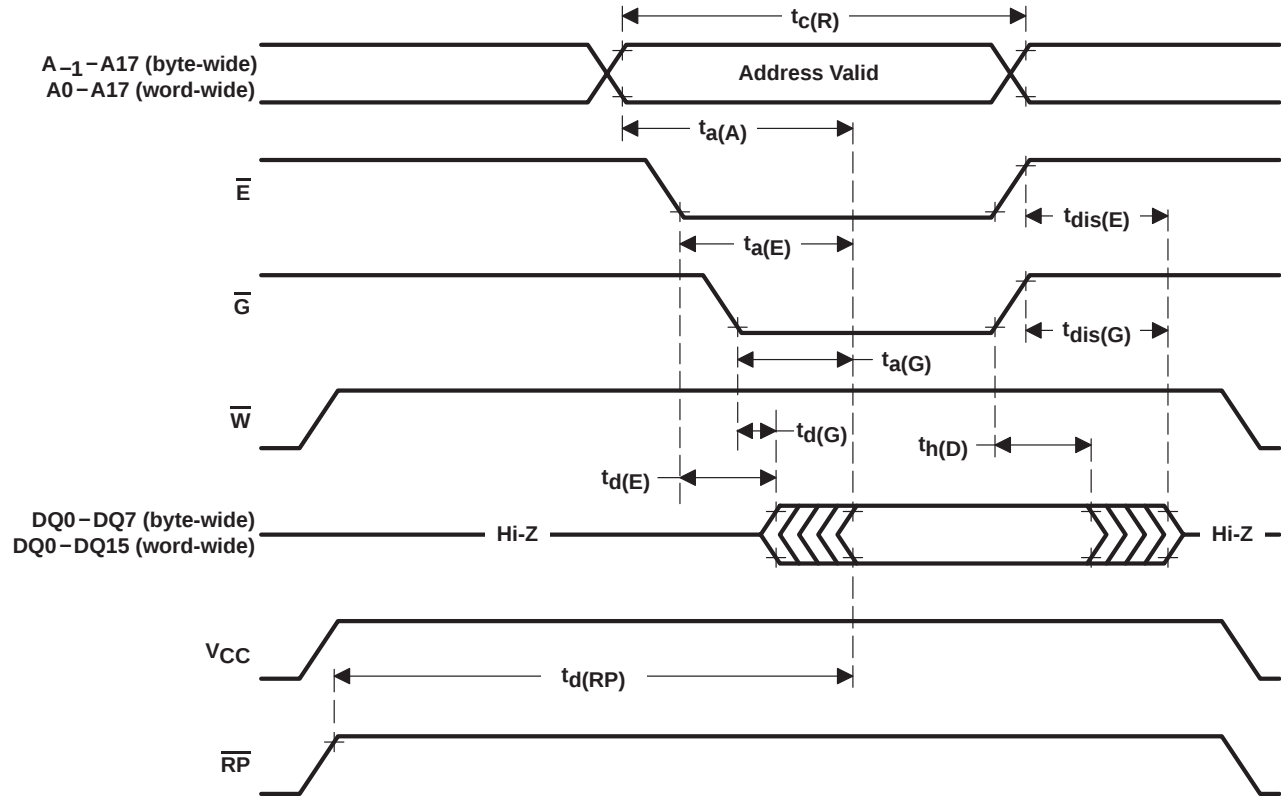
Figure 11. Read-Cycle Timing
