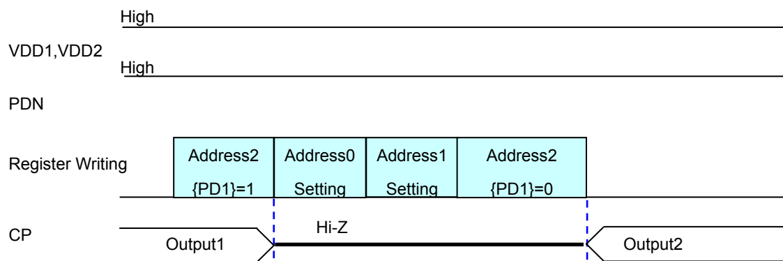
Frequency Change Sequence ({PD1} control)
