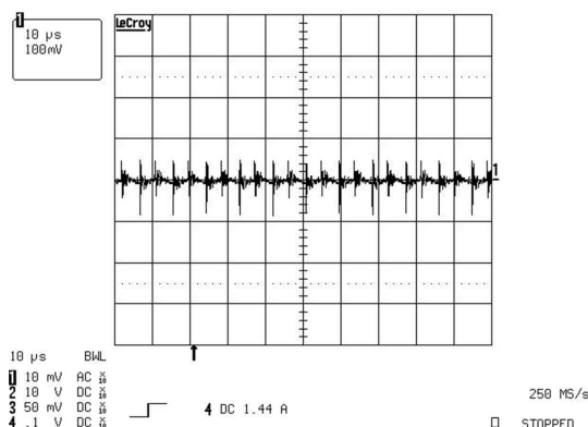
Figure 9-10. Output Voltage Ripple at Full Load (100 mV/div)
