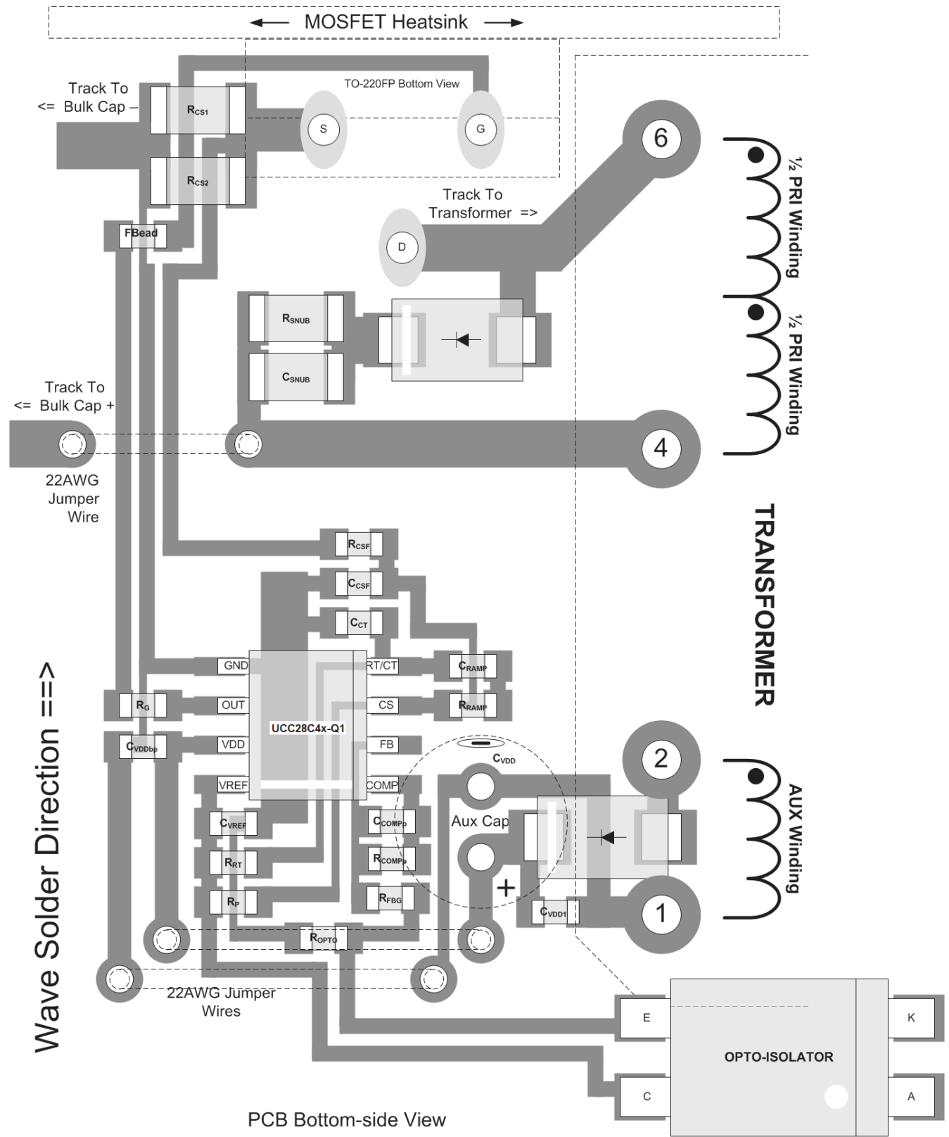
Figure 9-12. UCC28C4x-Q1 Layout Example
