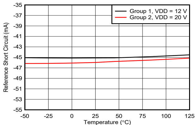
Figure 7-7. Reference Short-Circuit Current vs Temperature
