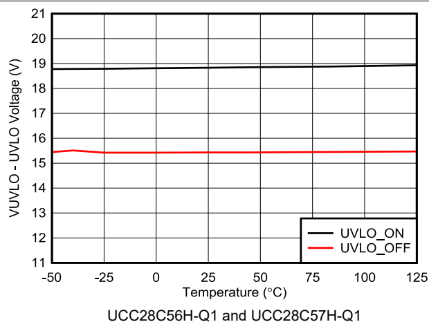
Figure 7-12. Undervoltage Lockout vs Temperature
