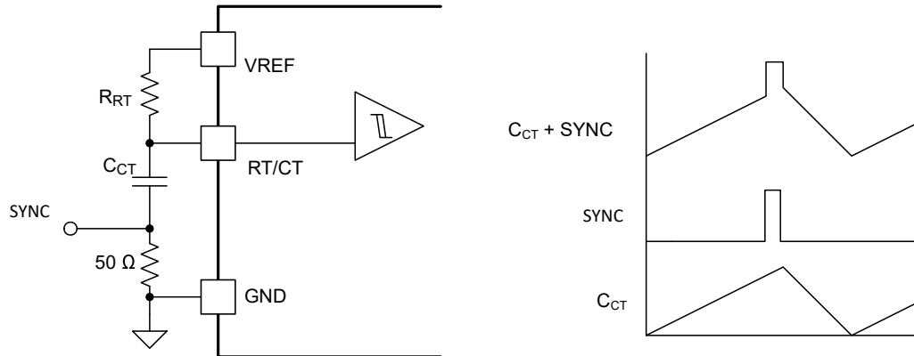
Figure 8-5. Oscillator Synchronization Circuit
