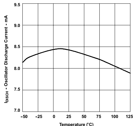
Figure 7-2. Oscillator Discharge Current vs Temperature
