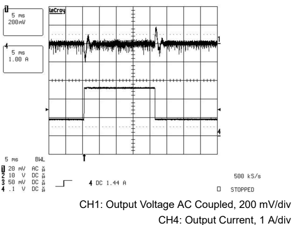
Figure 9-9. Output Voltage During 0.9-A to 2.7-A Load Transient
