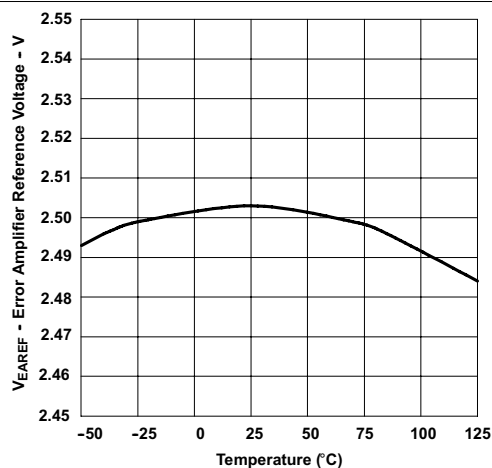
Figure 7-6. Error Amplifier Reference Voltage vs Temperature
