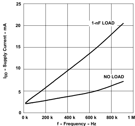
Figure 7-15. Supply Current vs Oscillator Frequency
