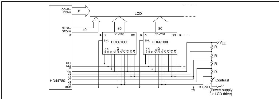
Figure 10 Example of Connection (1/8 Duty Cycle, 1/4 Bias)
