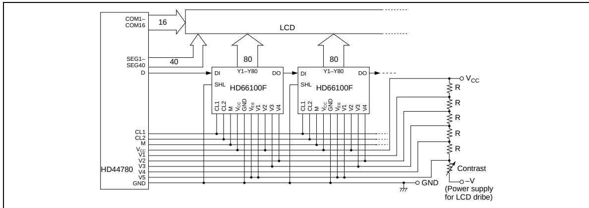
Figure 9 Example of Connection (1/16 Duty Cycle, 1/5 Bias)
