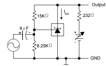
TEST CIRCUIT FOR VOLTAGE AMPLIFICATION
