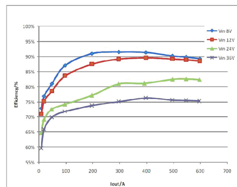
Efficiency @ Vout=5V
