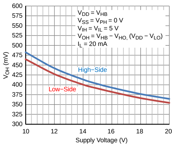
Figure 25. High-Level Output Voltage Deviation from the V_{BH} ( V_{DD} ) vs. Supply Voltage ( V_{DD} )
