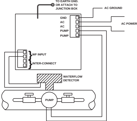
WIRING DIAGRAM FOR STAND ALONE APPLICATION
