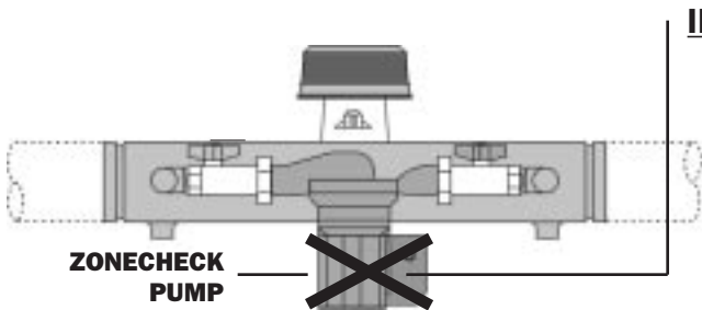
Incorrect Horizontal Installation
