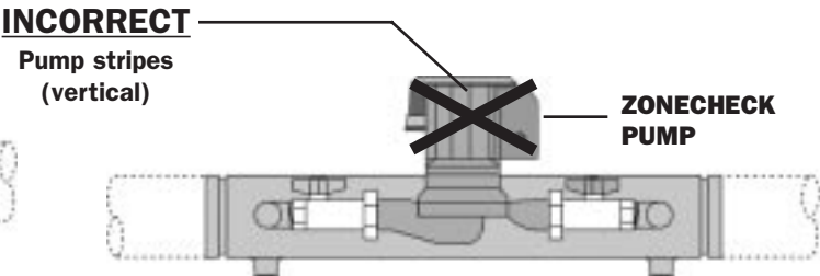
Incorrect Horizontal Installation
