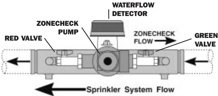
Correct Horizontal Installation
