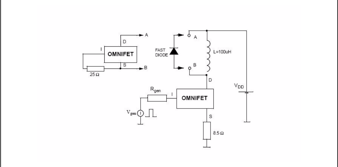
Figure 5. Test circuit for diode recovery times
