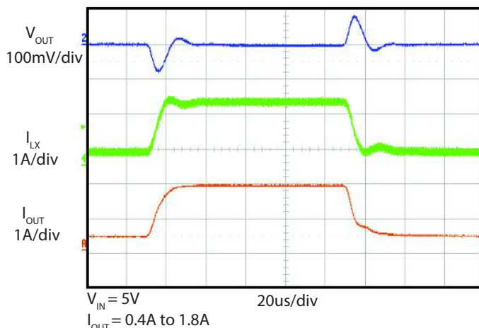
Transient Response ( V_{OUT}=1.5V , I_{OUT}=0.4A to 2A )
