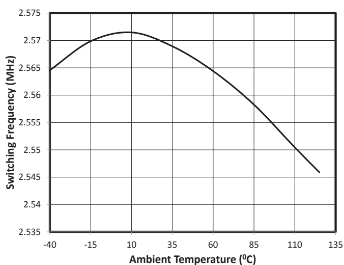
Switching Frequency Vs Temperature, V_{out}=1.8V
