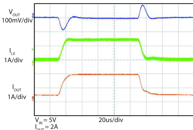
Transient Response ( V_{OUT}=3.3V , I_{OUT}=0.4A to 2A )
