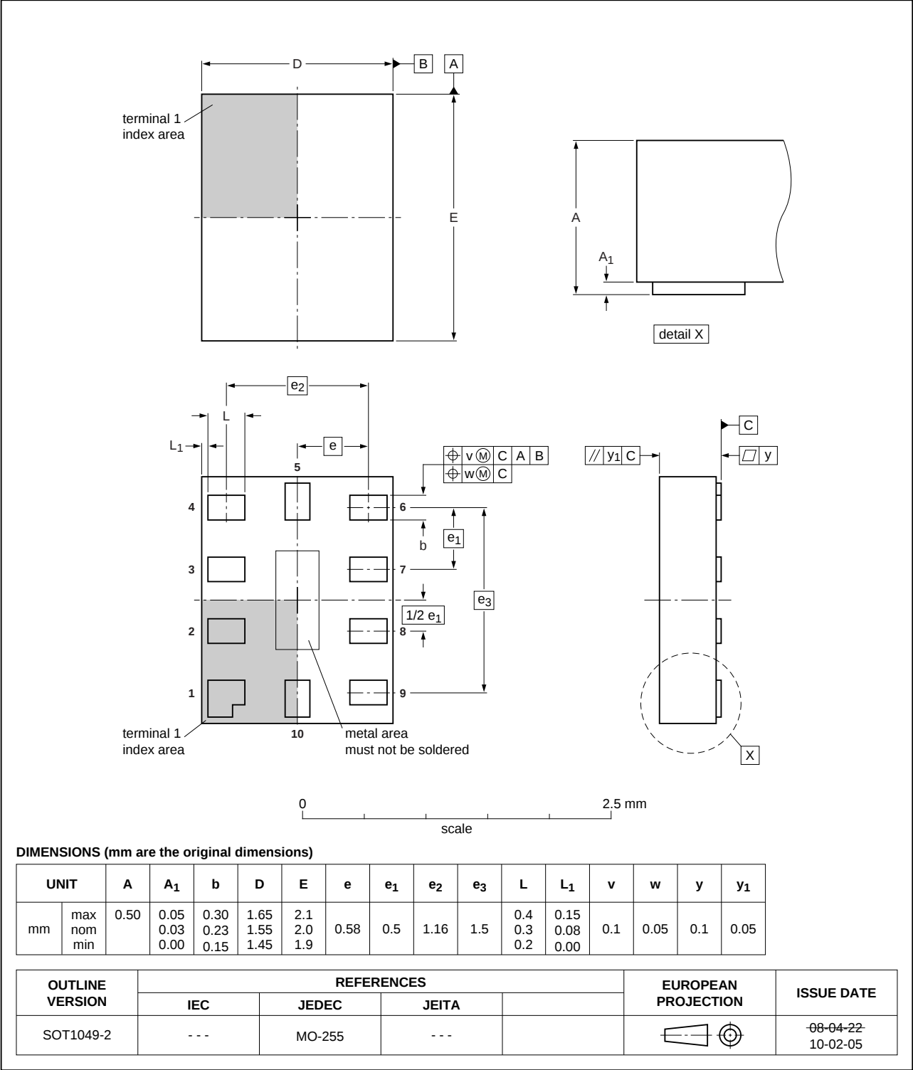
Fig 16. Package outline SOT1049-2 (XQFN10U)
