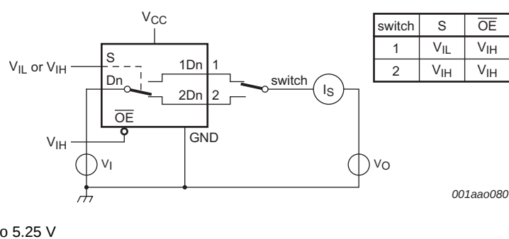
Fig 3. Test circuit for measuring OFF-state leakage current
