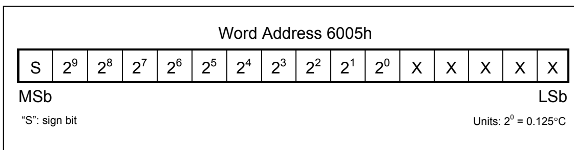
Figure 16. Temperature Register Format
