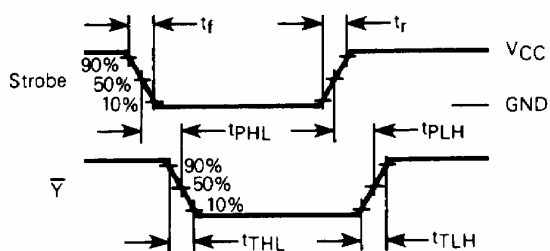
Figure 5. Switching waveforms
