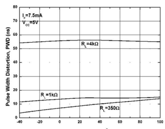
Fig 10 Pulse Width Distortion vs T_A
