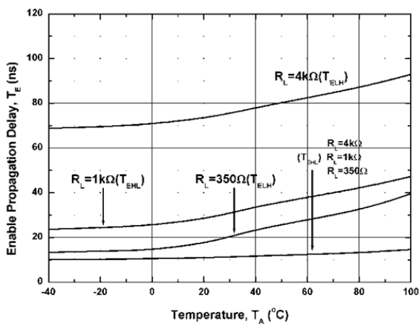
Fig 9 Enable Propagation Delay Time vs T_A
