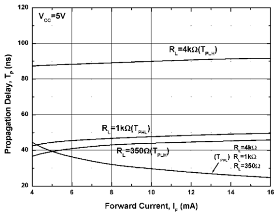
Fig 7 Propagation Delay Time vs Forward Current
