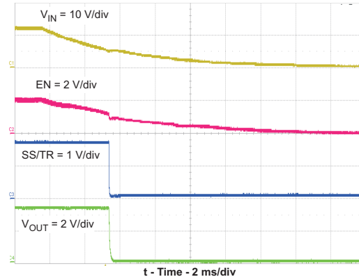
Figure 42. Shutdown With VIN (1.1-Ω Load)
