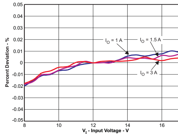
Figure 48. Line Regulation
