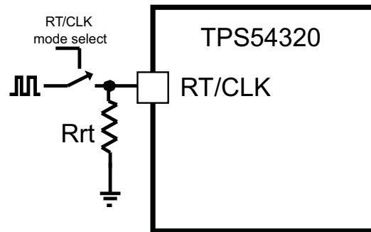
Figure 33. Works With Both RT Mode and CLK Mode
