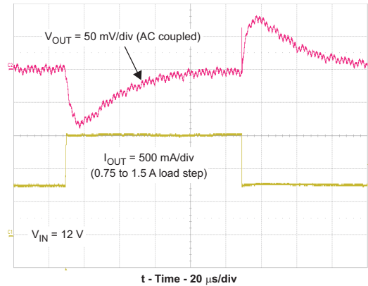
Figure 35. Load Transient
