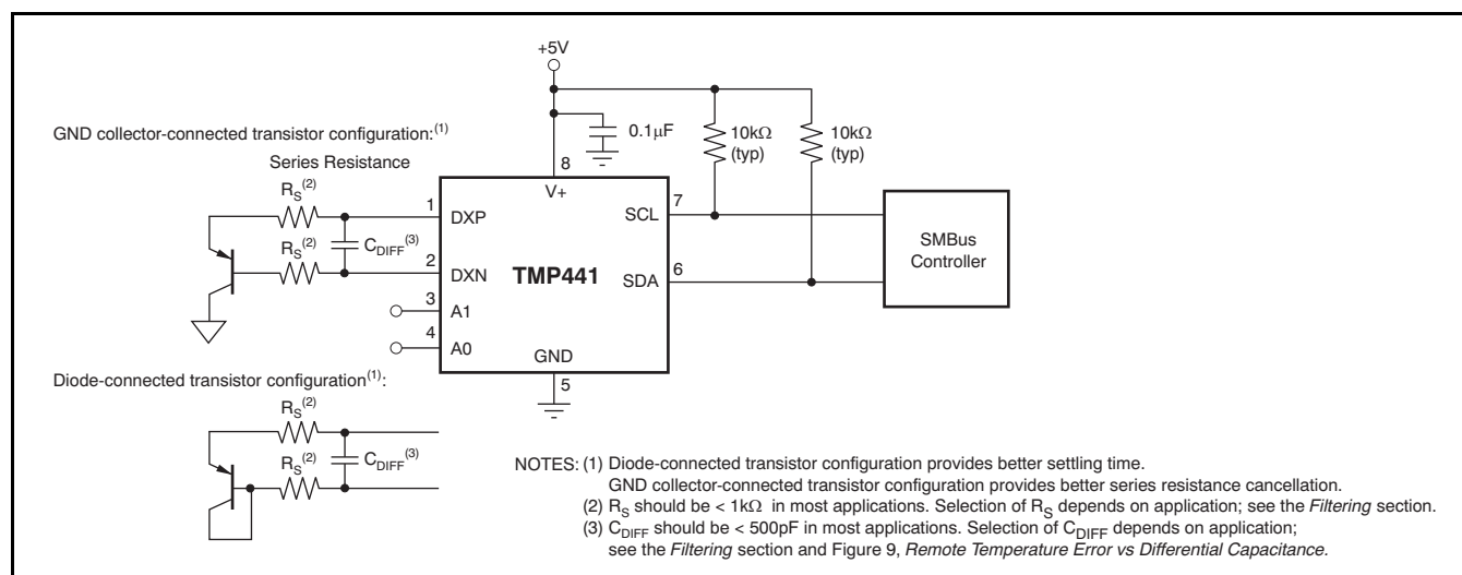
Figure 12. TMP441 Basic Connections
