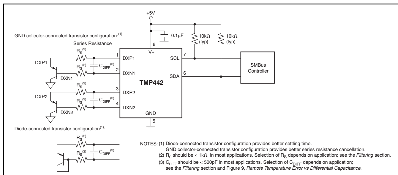
Figure 13. TMP442 Basic Connections
