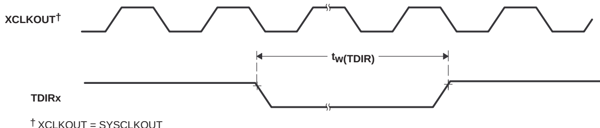
Figure 6–19. TDIRx Timing
