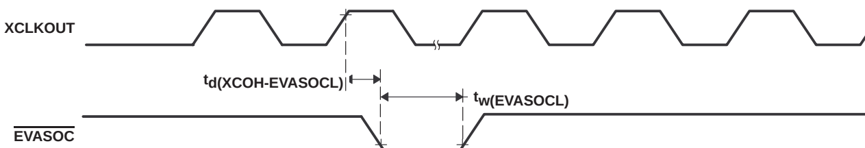
Figure 6–20. \overline{\text{EVASOC}} Timing
