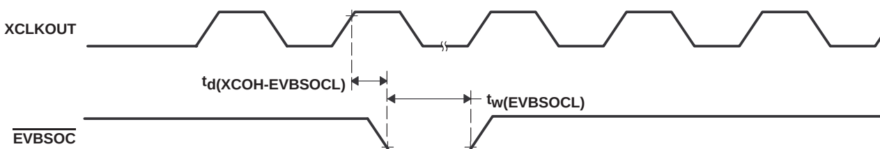
Figure 6–21. \overline{\text{EVBSOC}} Timing
