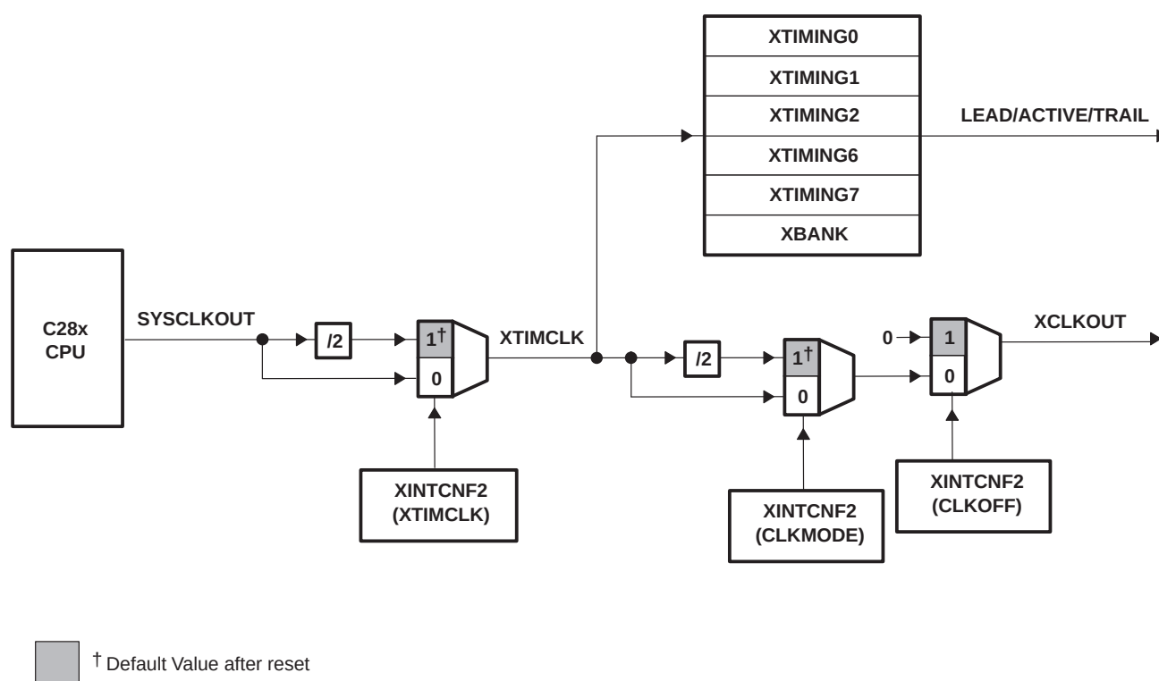
Figure 6–30. Relationship Between XTIMCLK and SYSCLKOUT
