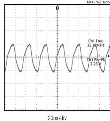
CLOCK OUTPUT DRIVER WITH 40pF LOAD
