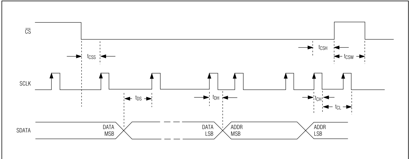
Figure 5. 3-Wire Timing Diagram
