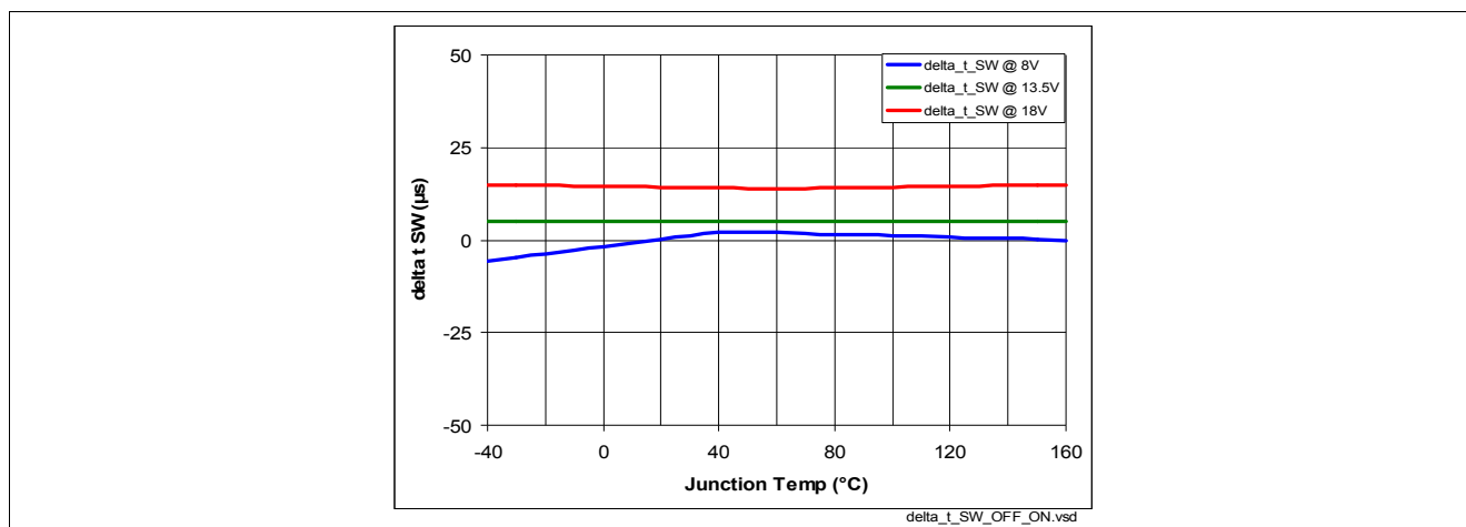
Figure 40 Turn ON / OFF matching \Delta t_{SW} = f(T_J; V_S) , R_L = 6 \Omega
