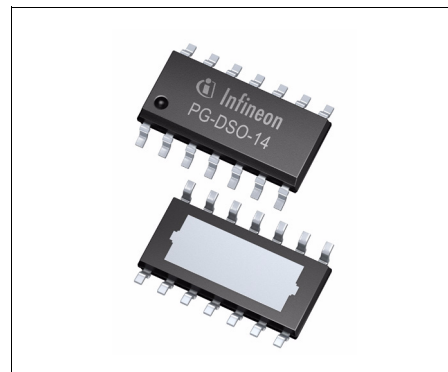
PG-DSO-14-40 EP
