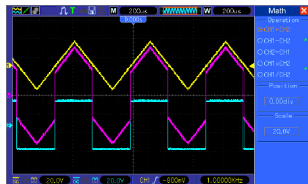
Math: CH1+CH2
