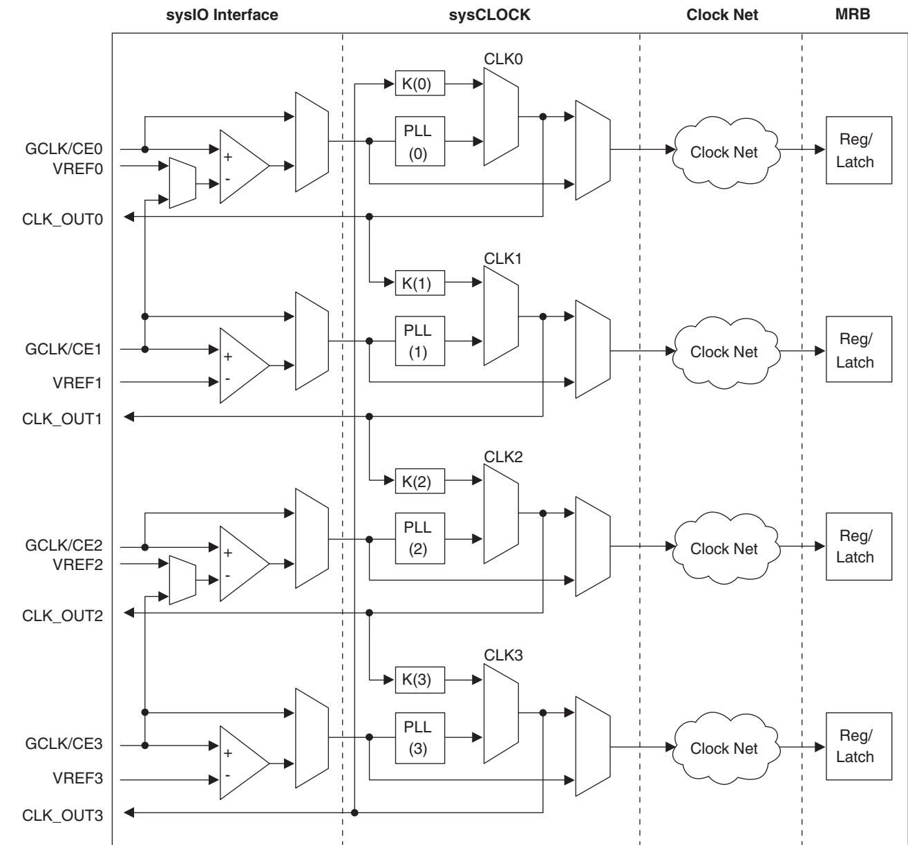
Figure 10. ispGDX2-256 CLOCK Network
