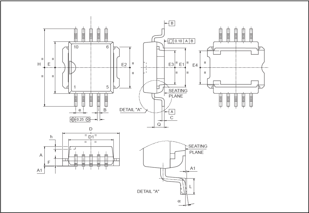
Figure 20. Package Dimensions
