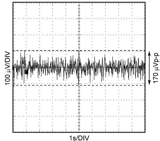
Figure 14. 0.1–10 Hz Noise
