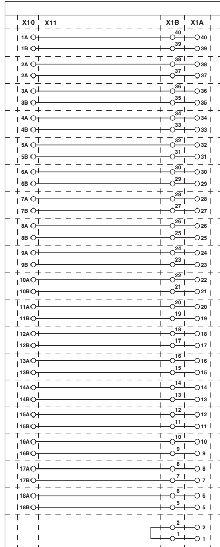
Circuit diagram
