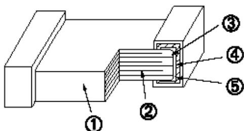
Construction of MLCC
