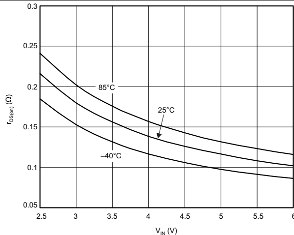
Figure 5. r_{DS(on)} NMOS versus V_{IN}
