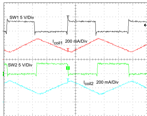
Time base – 100 ns/Div V_{IN} = 3.6 V V_{OUT1} = 1.575 V V_{OUT2} = 1.8 V I_{OUT1} = I_{OUT2} = 200 mA
