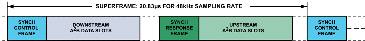
Figure 3. A²B Superframe
