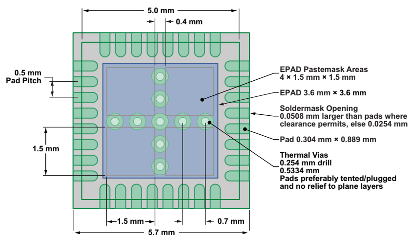
Figure 38. Transceiver Footprint
