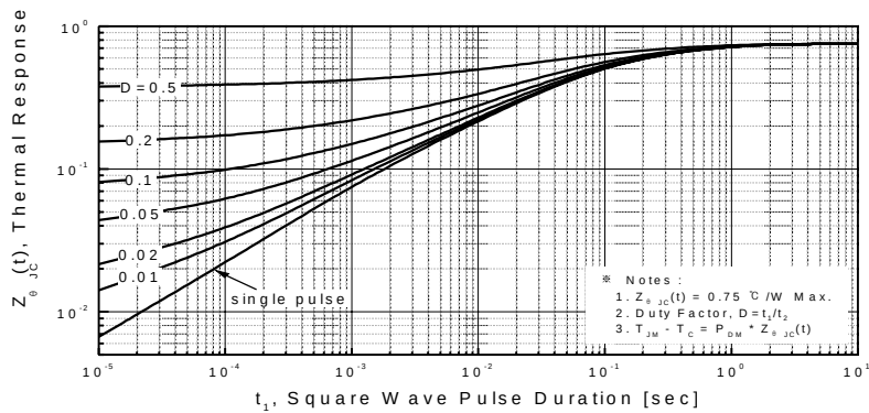
Figure 11. Thermal Response
