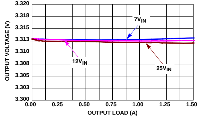
FIGURE 10. V_{OUT} REGULATION vs LOAD, 500kHz 3.3V _{OUT}
