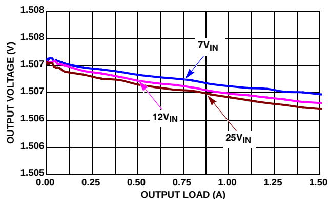
FIGURE 7. V_{OUT} REGULATION vs LOAD, 500kHz 1.2V OUT
