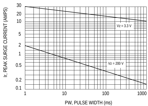
Fig. 4 Peak Surg Current versus Pulse Width
