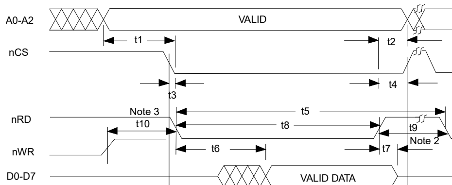
FIGURE 8-6: NON-MULTIPLEXED BUS, 80XX-LIKE CONTROL SIGNALS; READ CYCLE
