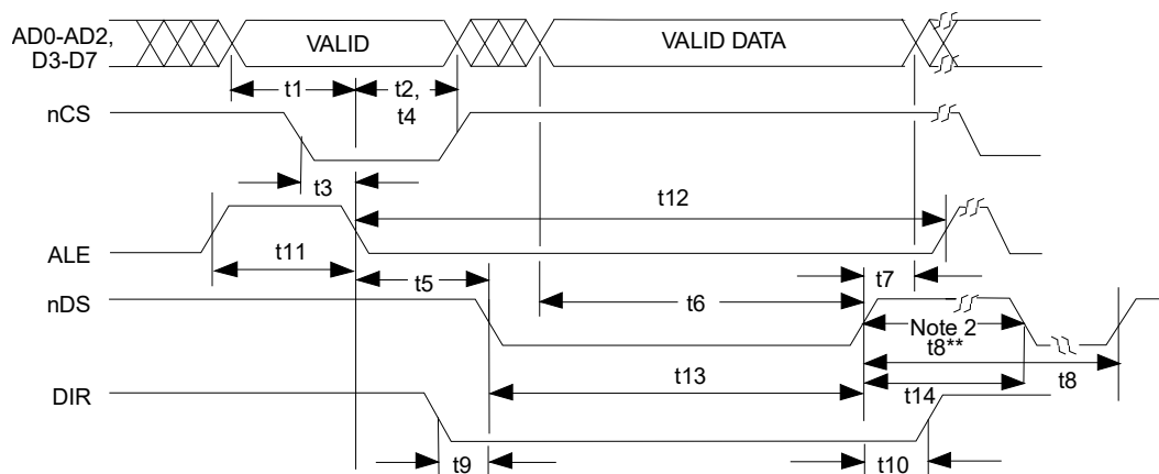
FIGURE 8-3: MULTIPLEXED BUS, 68XX-LIKE CONTROL SIGNALS; WRITE CYCLE
