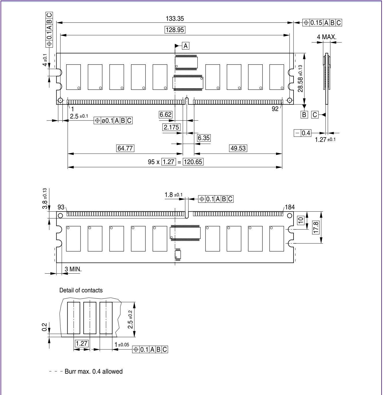
Package Outlines – Raw Card B HYS72D64320GBR-[5/6]-C (2 Ranks x8)
