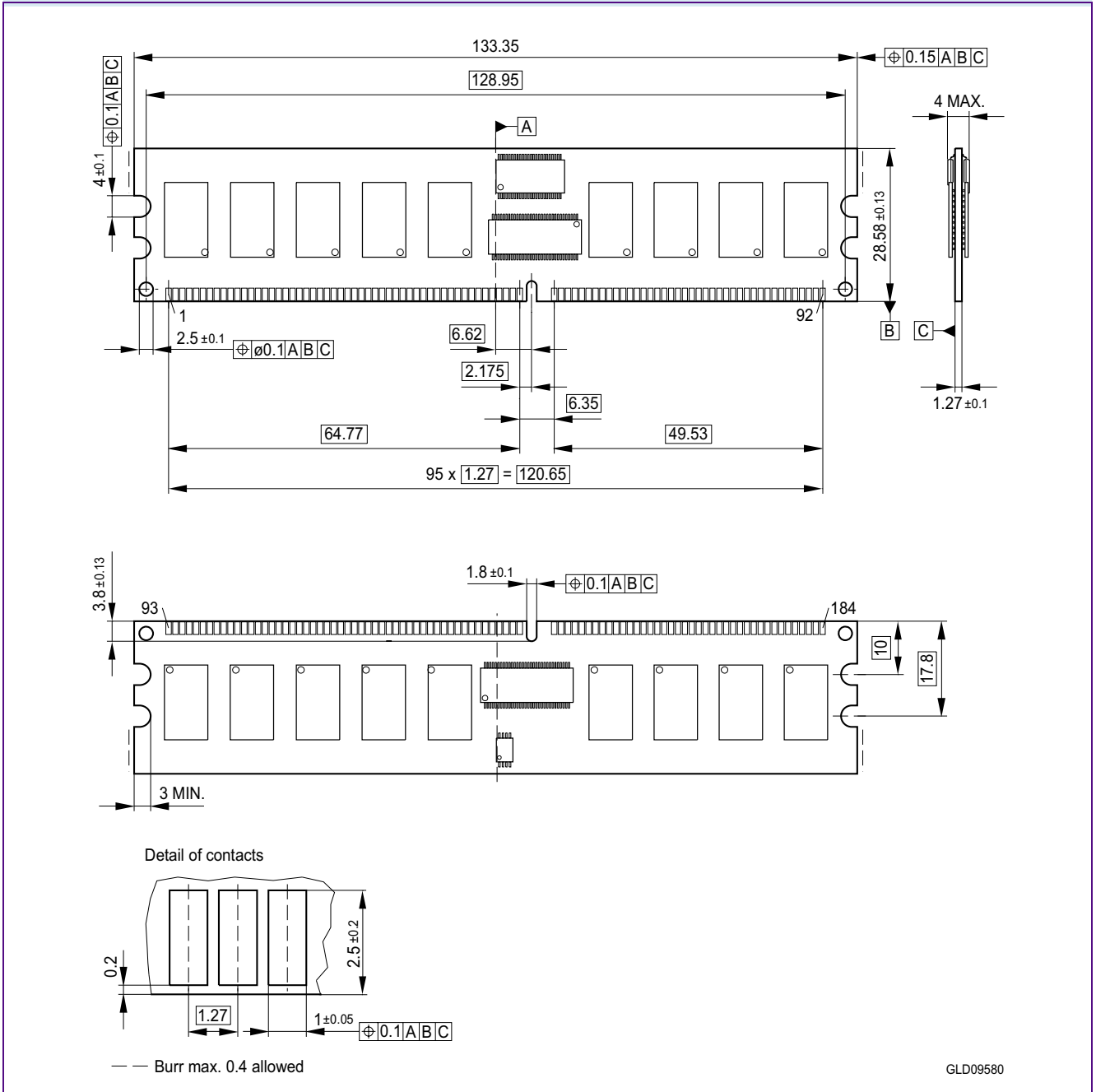
Package Outlines – Raw Card C HYS72D64300[G/H]BR-[5/6/7]-C (1 Rank × 4)
