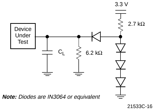
Figure 11. Test Setup
