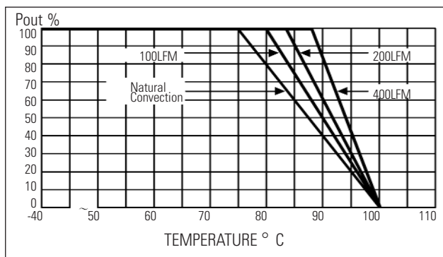
MODEL 100HFS Dual - 5V Output
