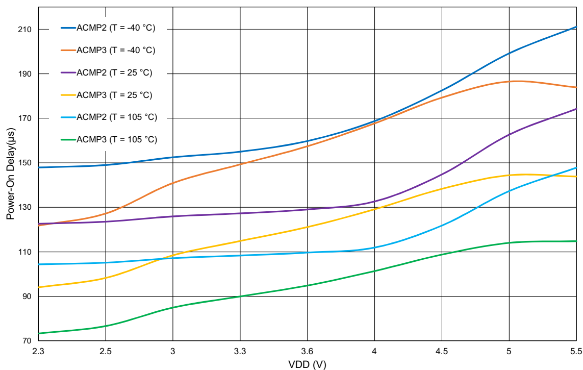
Figure 62: ACMPxL Power-On Delay vs. V_{DD}
