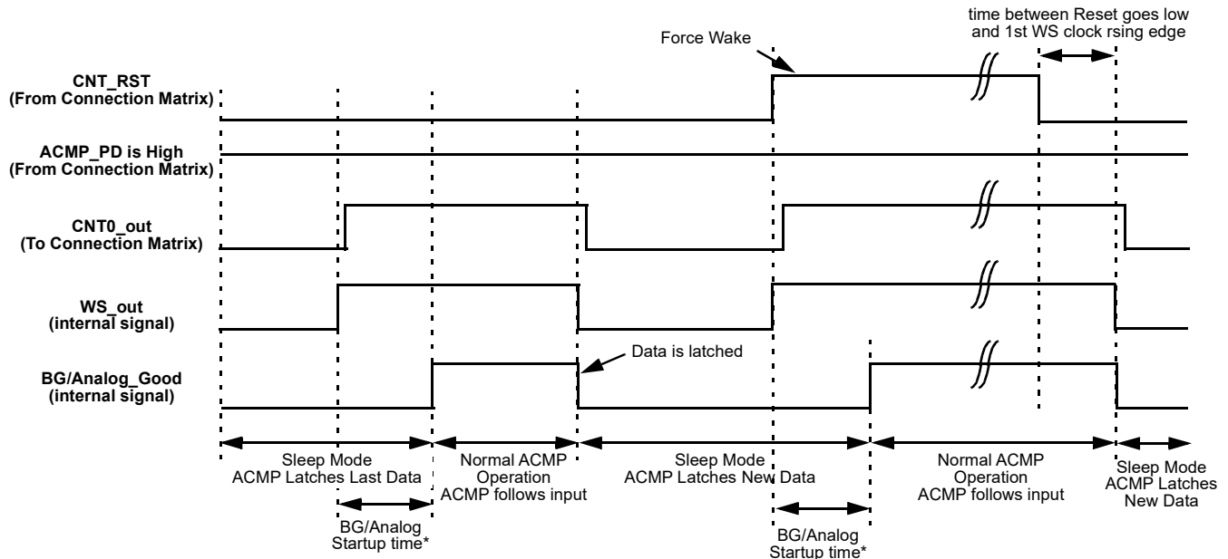
Figure 51: Wake and Sleep Timing Diagram, Normal Wake Mode, Counter Reset is Used
