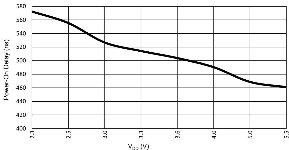
Figure 81: Oscillator1 Maximum Power-On Delay vs. V_{DD} at T = 25^{\circ}\text{C} , \text{OSC1} = 2.048\text{ MHz}
