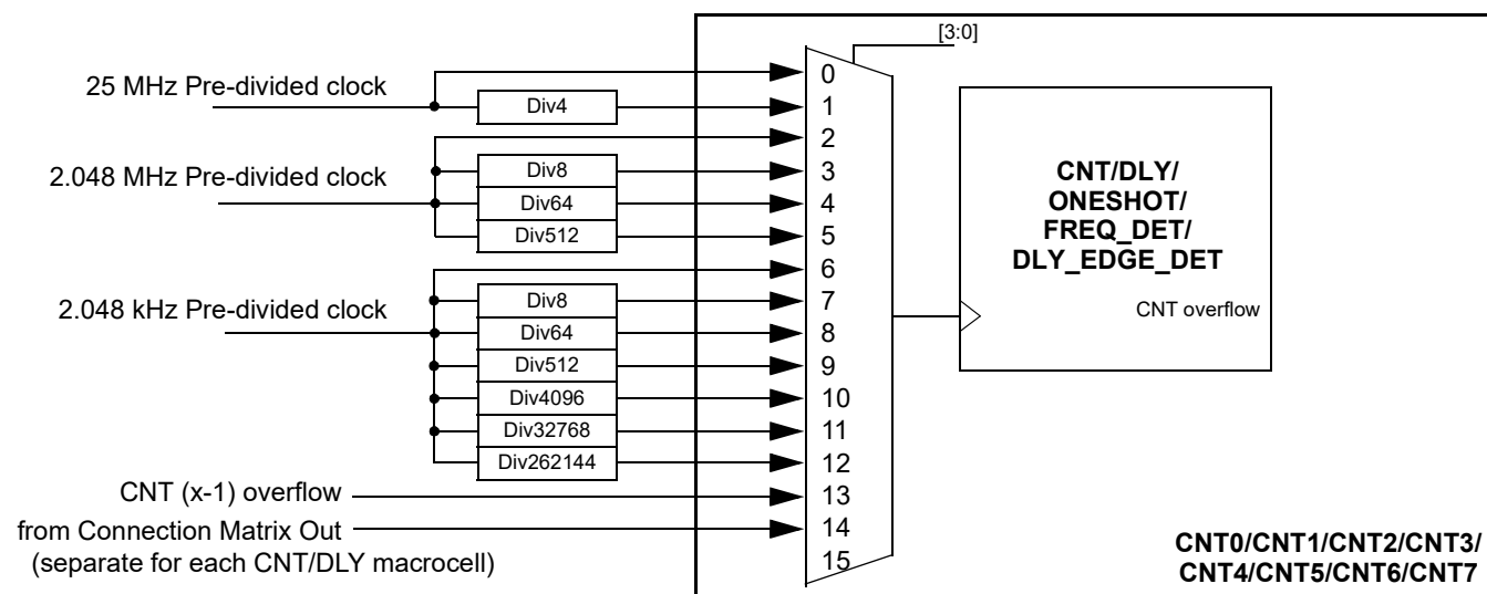
Figure 78: Clock Scheme
