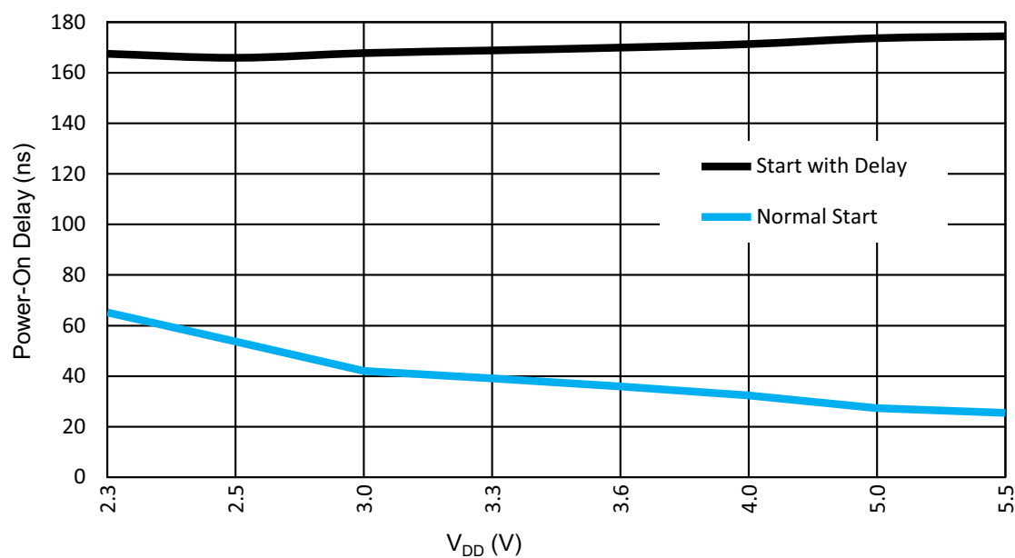
Figure 82: Oscillator2 Maximum Power-On Delay vs. V_{DD} at T = 25^{\circ}\text{C} , \text{OSC2} = 25\text{ MHz}
