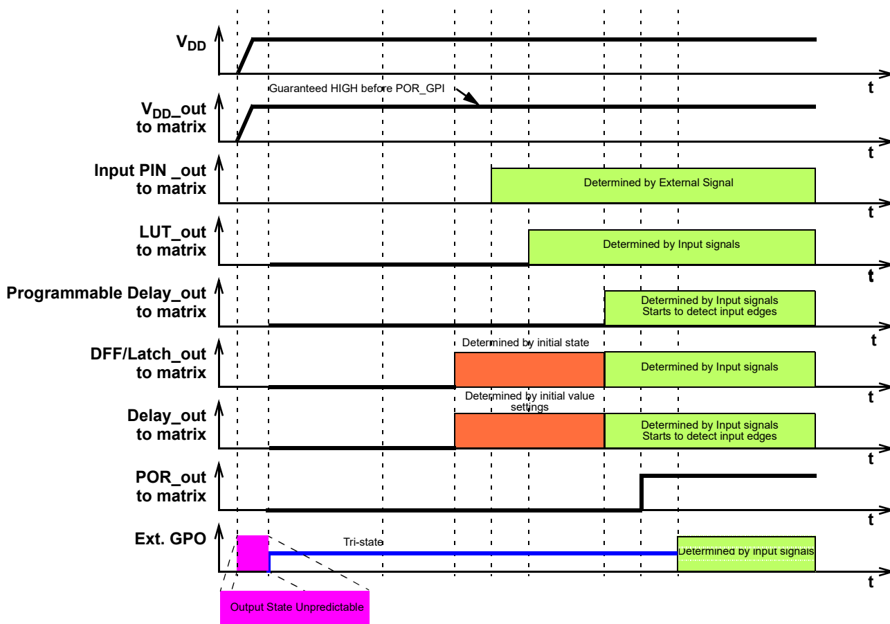
Figure 88: Internal Macrocell States during POR Sequence
