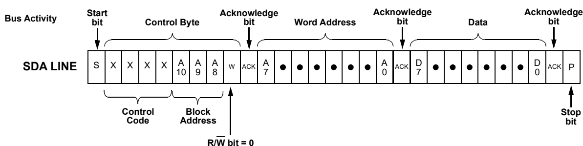
Figure 92: Byte Write Command, R/\bar{W} = 0
