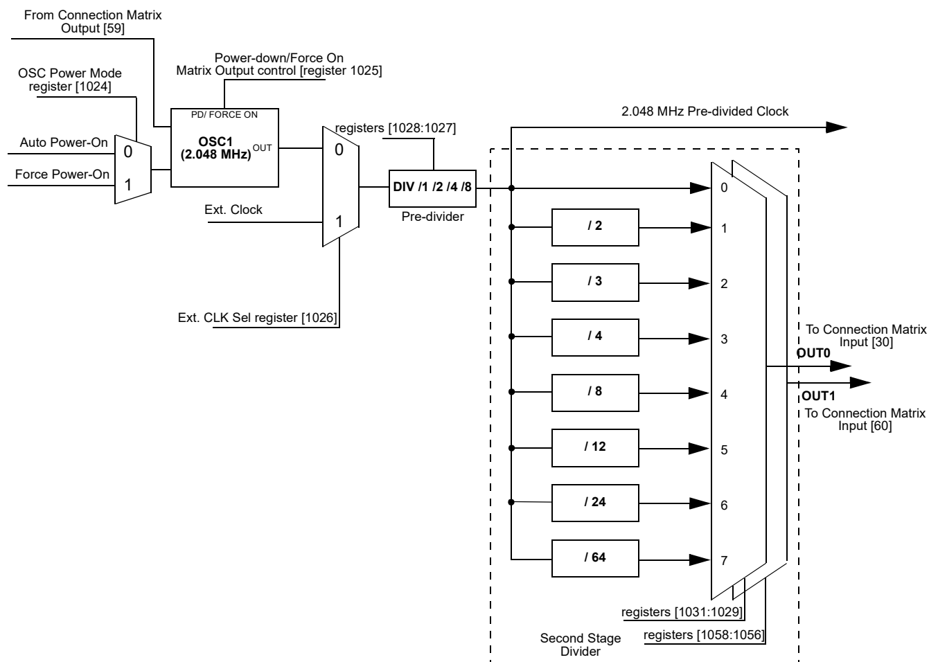
Figure 76: Oscillator1 Block Diagram
