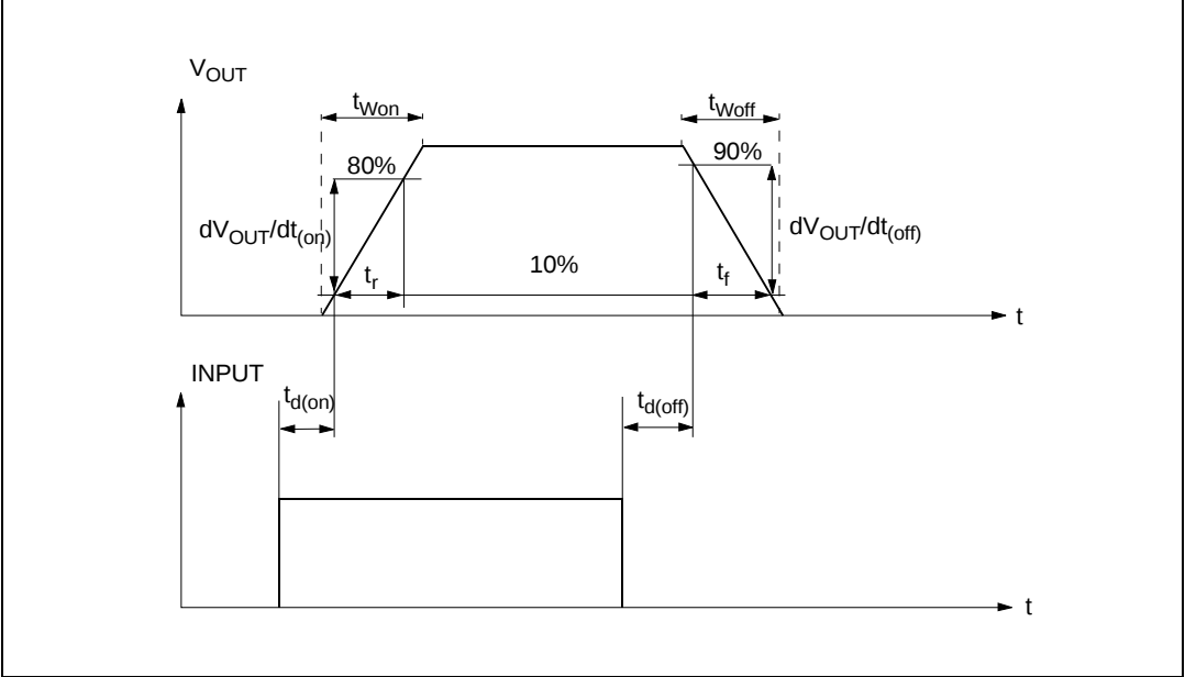
Figure 6. Switching characteristics
