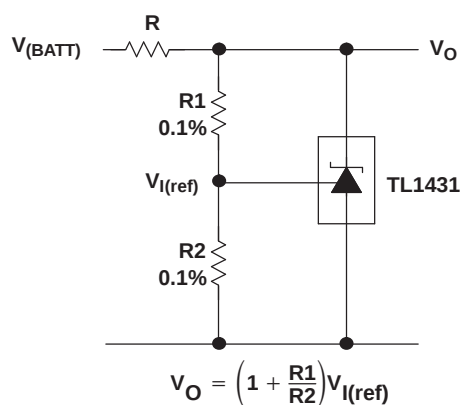
Figure 16. Shunt Regulator
