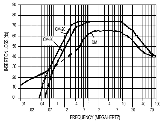
INSERTION LOSS 1306 SERIES
