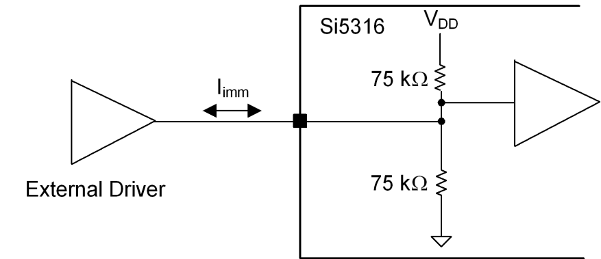
Figure 3. Three-Level (3L) Input Pins (No External Resistors)
