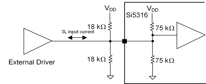
Figure 4. Three-Level Input Pins (Example with External Resistors)
