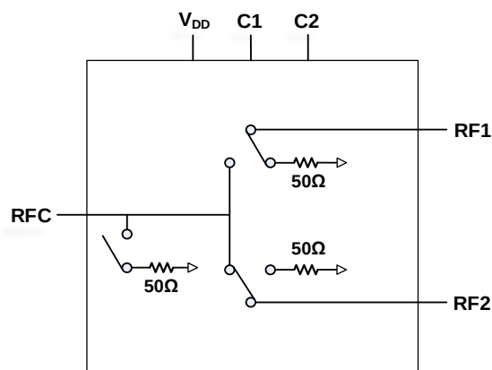
Figure 1. Block Diagram
